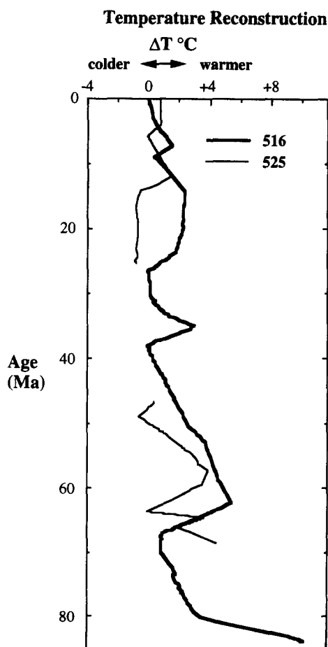
FIG. 9. Relative change in sea surface temperatures reconstructed from the corrected data for sites 516 and 525. To calculate the temperatures, we use the model \delta^{18}\text{O}_{\text{seawater}} (Fig. 3) and the \delta^{18}\text{O} -temperature relationship from O'Neil et al. (1969), adjusted for the fractionation factor between \text{CO}_2 and water from Friedman and O'Neil (1977). For site 516, we use the calculation with the higher recrystallization rate ( \alpha = 0.004 ).
