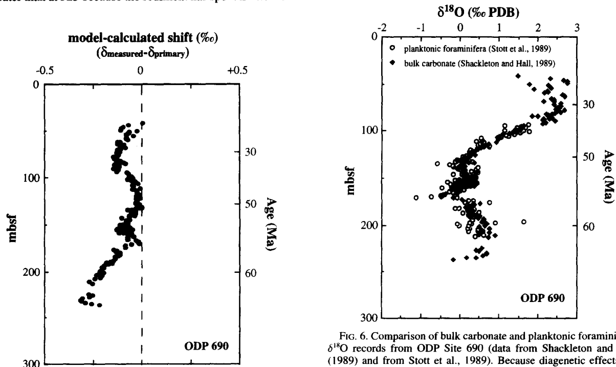
FIG. 5. Model-calculated shifts for bulk carbonate from ODP Site 690. Details of the model calculations are described in the text.
